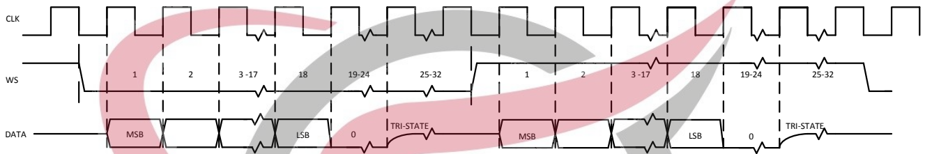
Figure 7: Timing Diagram
